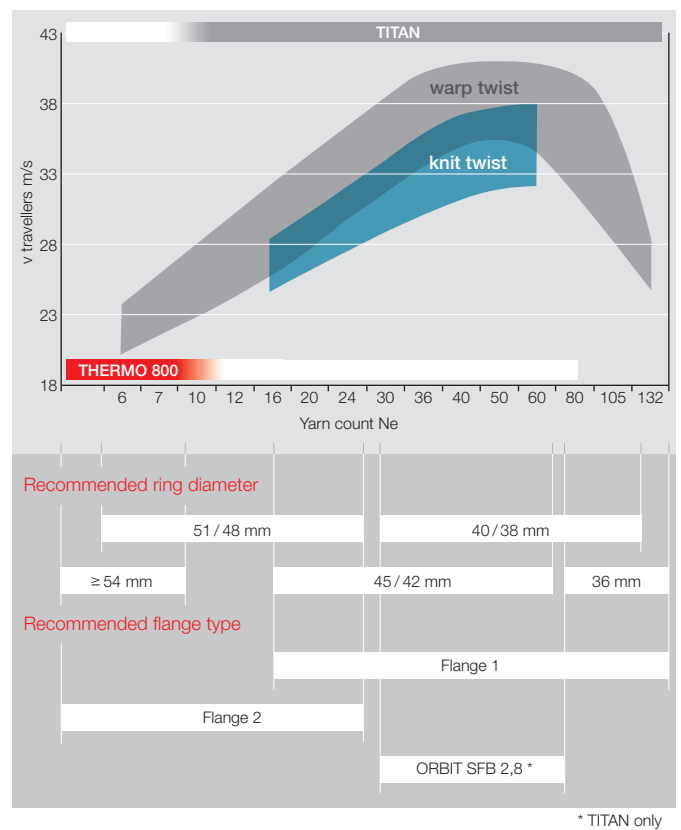
The THERMO 800 spinning ring is recommended especially for spinning core yarns for sewing threads and Denim yarns.
