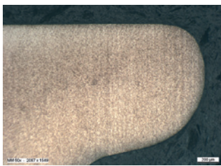
Micro structure of the THERMO 800 rings.
