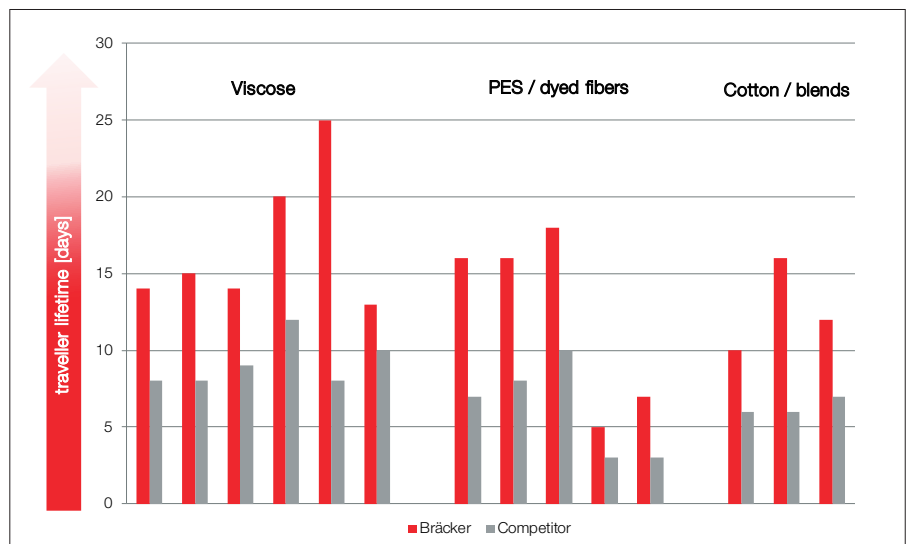
Traveller lifetime STARLET plus vs. competitor Ne 30/1 - 40/1; 17'000 - 18'000 rpm
